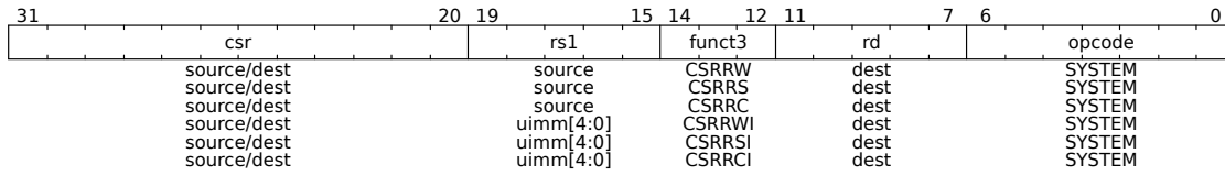
Figure 105: Zicsr Instructions
