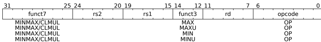
Figure 98: Comparison Instructions
