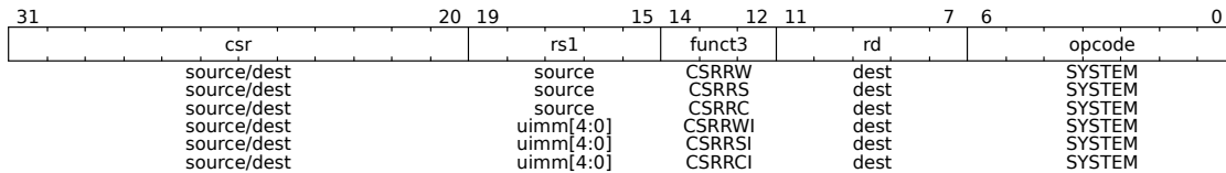
Figure 82: Zicsr Instructions
