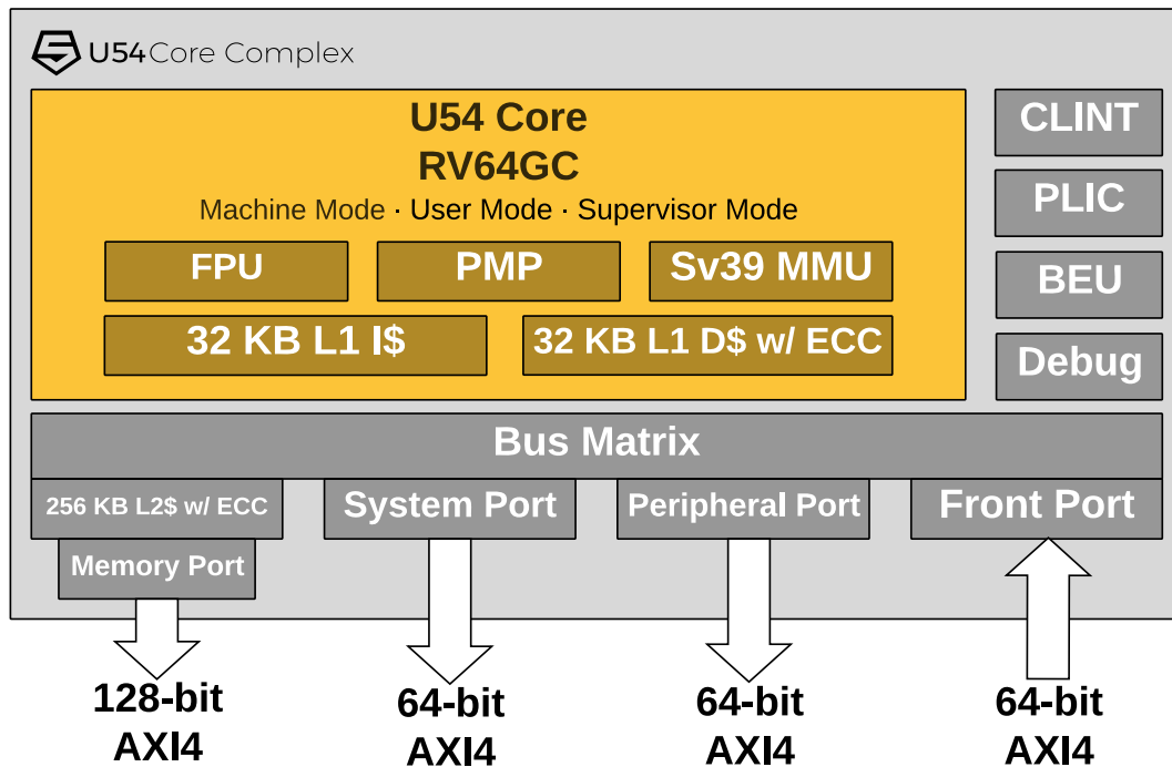
Figure 1: U5 Series Block Diagram
