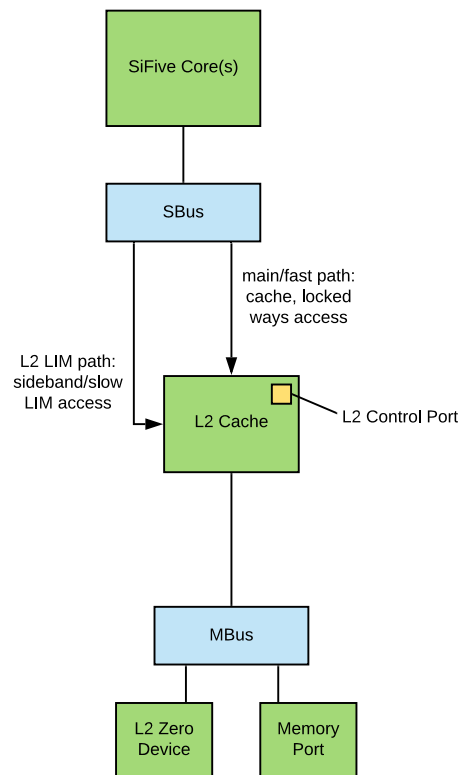
Figure 106: Difference between L2 LIM and L2 Zero Device
