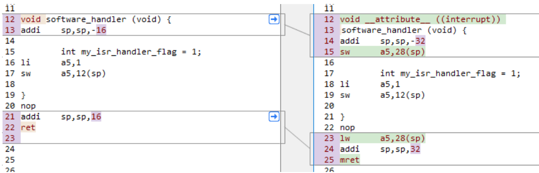
Figure 102: CLINT Interrupt Attribute Example
