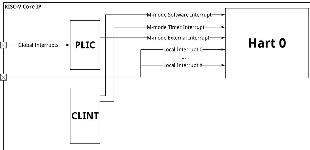
Figure 98: S76 Core Complex Interrupt Architecture Block Diagram
