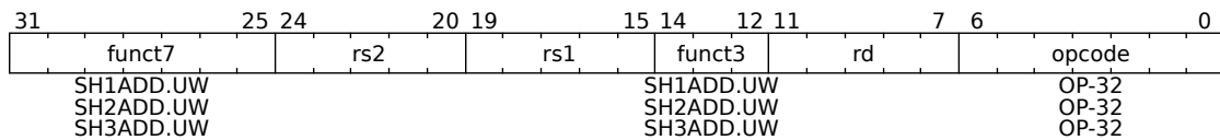
Figure 53: Address Calculation Instructions (cont.)
