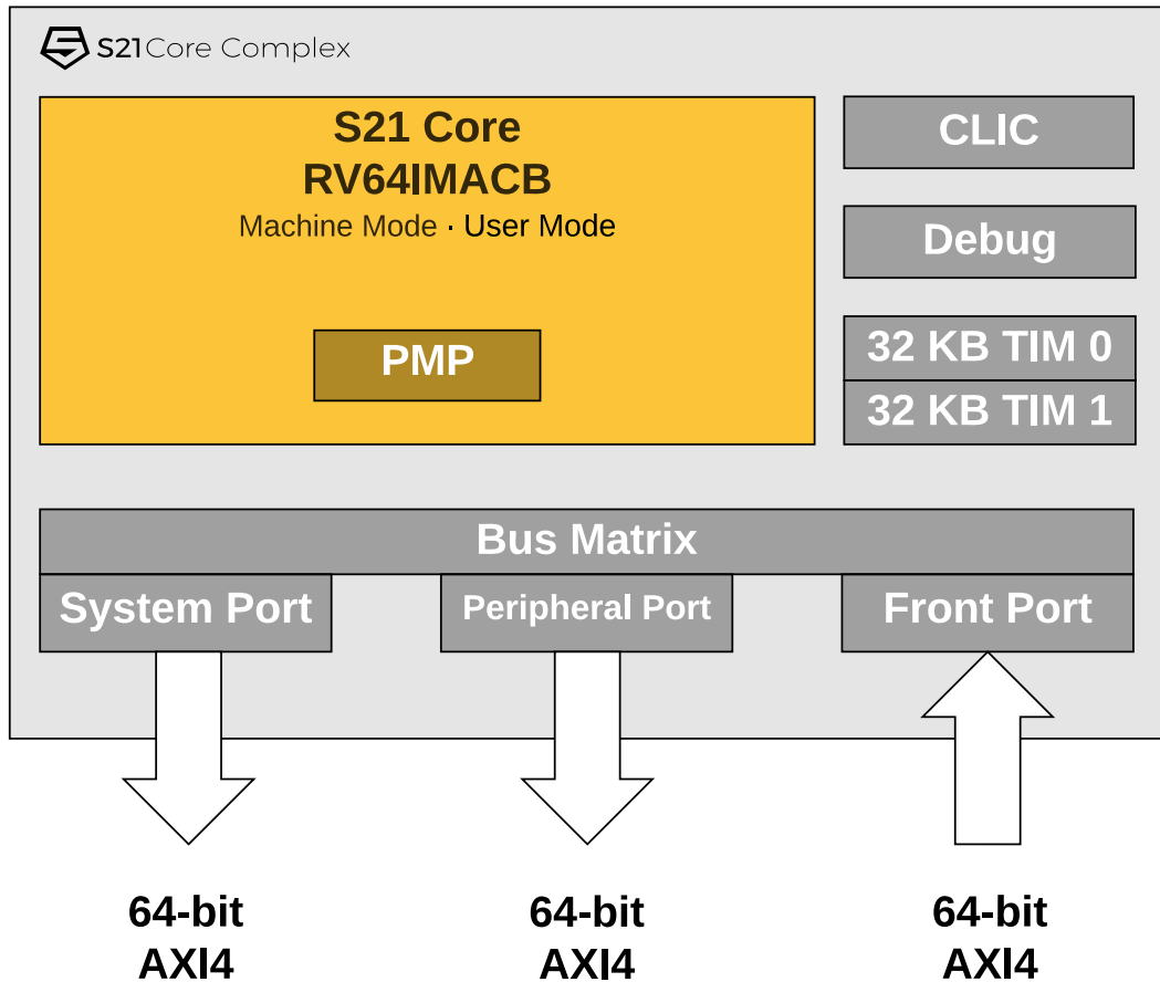
Figure 1: S2 Series Block Diagram
