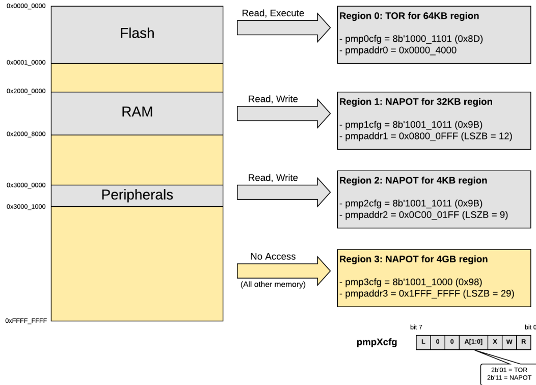
Figure 6: PMP Example Block Diagram
