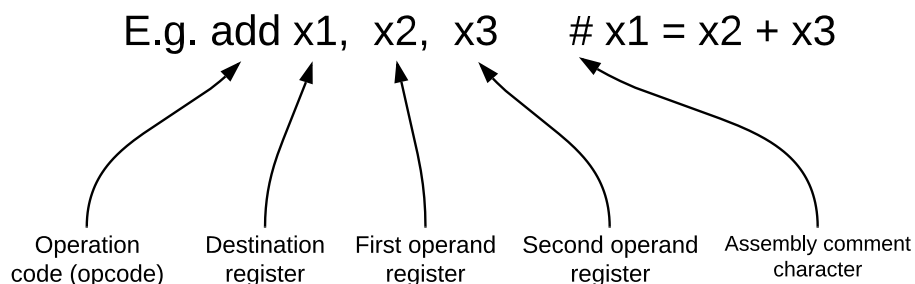
Figure 72: RISC-V Assembly Example
