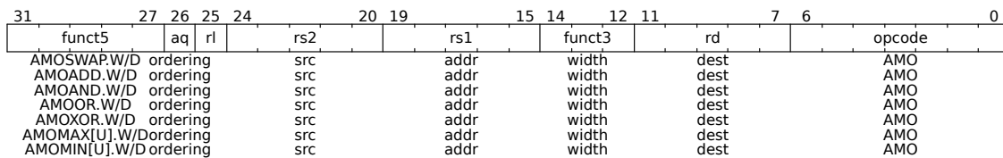
Figure 27: Atomic Memory Operations
