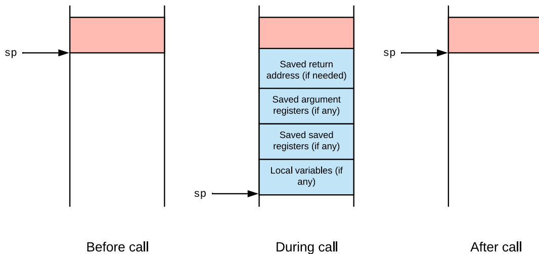
Figure 75: Stack Memory during Function Calls
