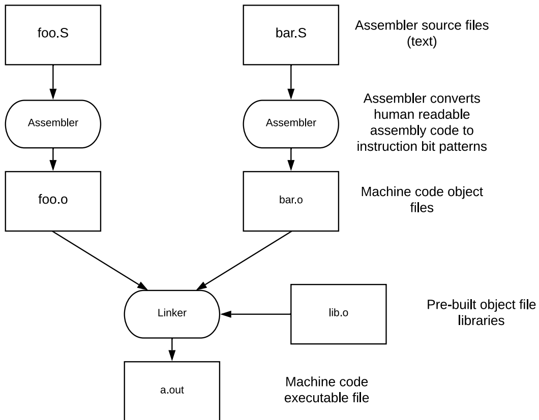
Figure 73: RISC-V Assembly to Machine Code
