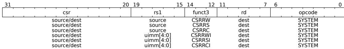
Figure 55: Zicsr Instructions
