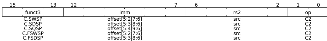
Figure 39: Stack-Pointed-Based Stores
