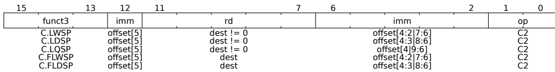
Figure 38: Stack-Pointed-Based Loads
