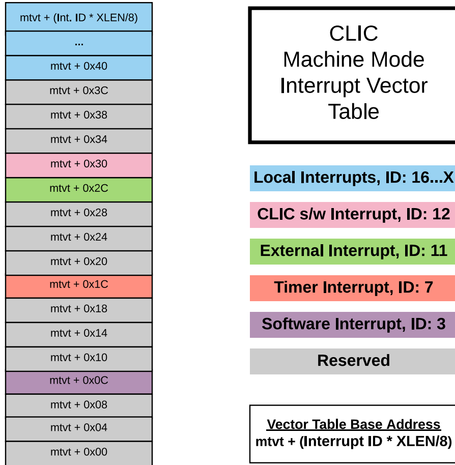
Figure 74: CLIC Interrupts and Vector Table
