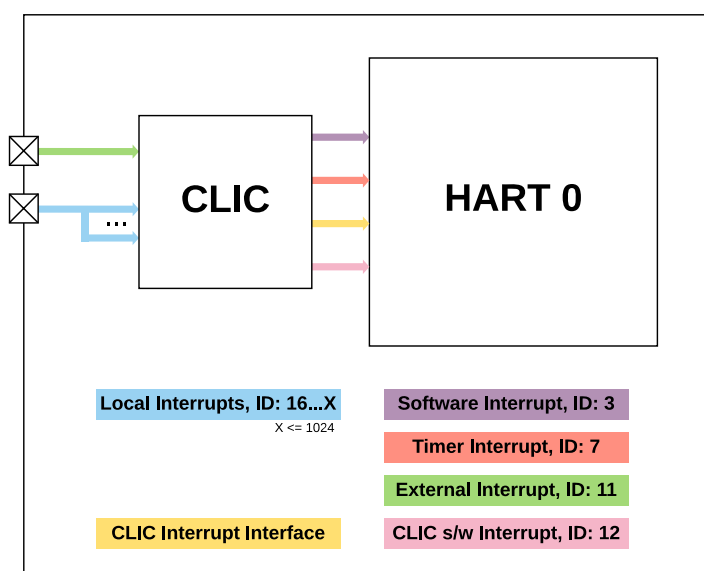
Figure 73: CLIC Block Diagram
