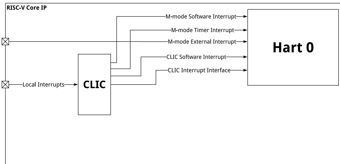
Figure 72: E21 Core Complex Interrupt Architecture Block Diagram
